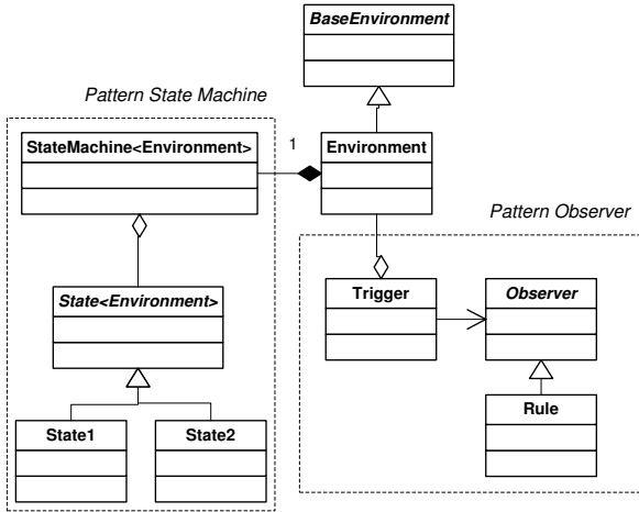
Figure 2. Kernel Architecture
