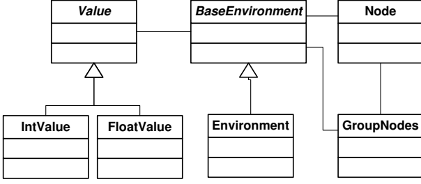
Figure 4. Network Structure
